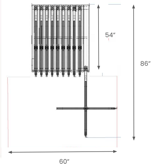
TOP VIEW ( Required floor space) Space required with panels open
