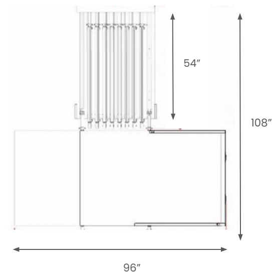
TOP VIEW ( Required floor space) Space required with panels open
