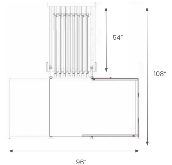
TOP VIEW ( Required floor space) Space required with panels open
